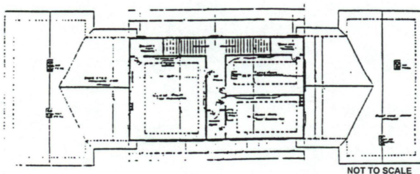
DESIGN NO. 17 -- SECOND FLOOR PLAN -- COUNTY TRAINING SCHOOL --GROUPED
