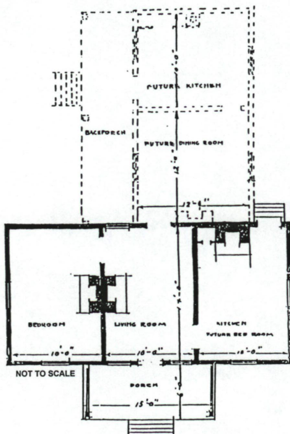
THREE ROOM COTTAGE DOTTED LINES SHOWS FUTURE ADDITIONS SCALE: 1/4" = 1'-0" DESIGN NO. 16 FLOOR PLAN, TEACHER'S HOME -THREE ROOMS,
