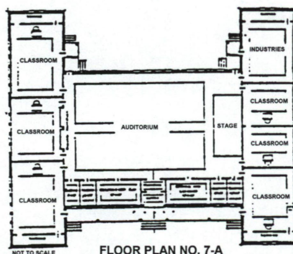
FLOOR PLAN NO. 7-A SEVEN TEACHER COMMUNITY SCHOOL (to face north or south only)
