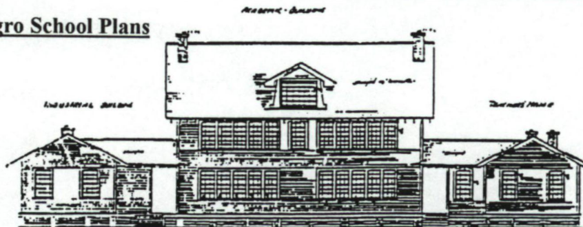
DESIGN NO. 17 -- A COUNTY TRAINING SCHOOL -- GROUPED
